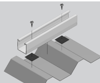
Detail ValkPitched - Trapezoidal
