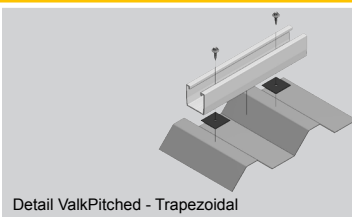
Detail ValkPitched - Trapezoidal
